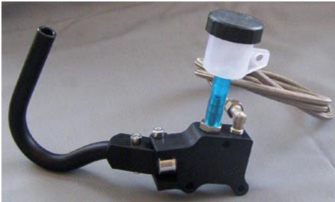
Hand clutch left hand
